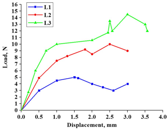
Fig. 10 Load vs displacement
