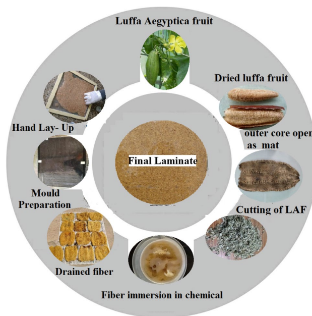
Fig. 1 Composite laminates fabricated in the present study
